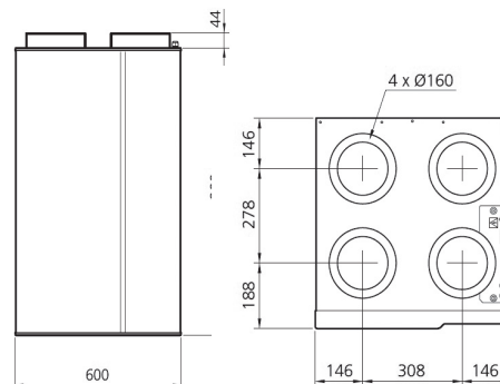
NIBE ERS 10-400/10-500/GV-HR 120-400
