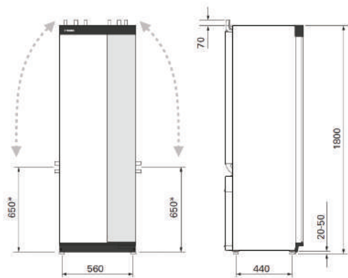
NIBE S1255
