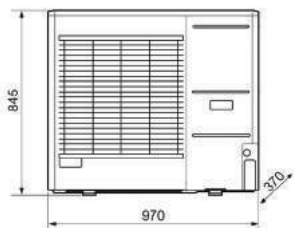
NIBE AMS 10-12
