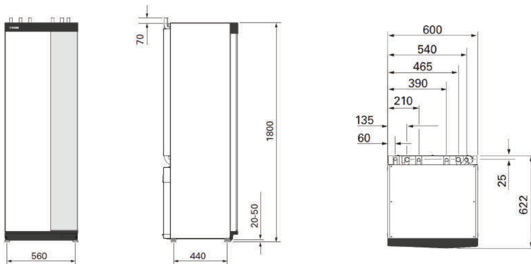
NIBE VVM S320
