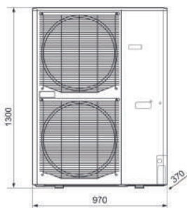
NIBE AMS 10-16
