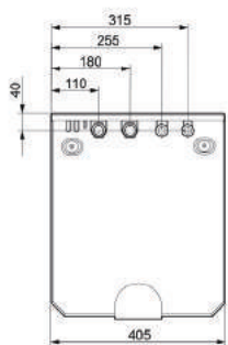
NIBE HBS
