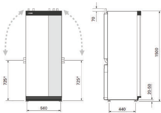
NIBE S1155
