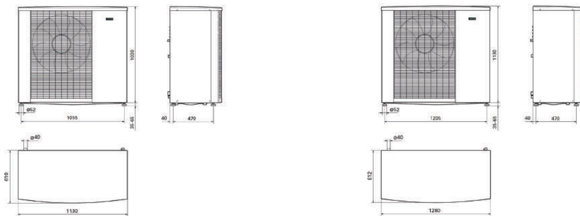
NIBE F2120-8
