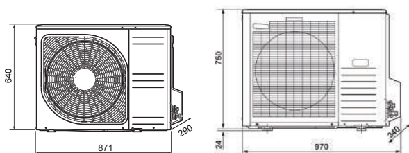
NIBE AMS 10-6
